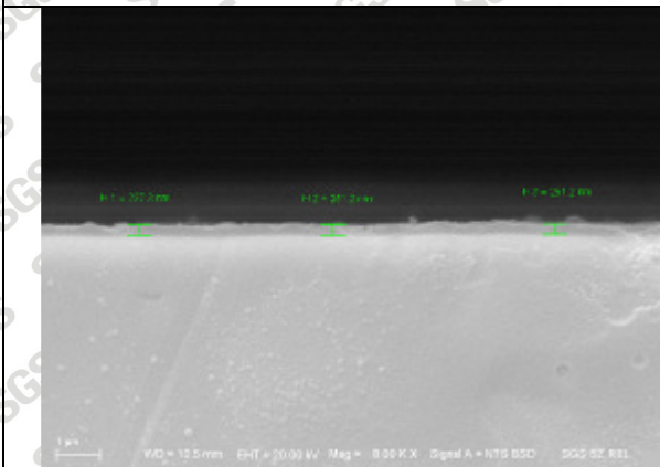
Fig.47 SEM observation – Black-8000X
