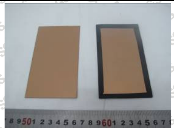
Fig.22 Reference sample Tested sample PVD Rose Gold Colored Stainless Steel Sheets Neutral Salt Spray Test
