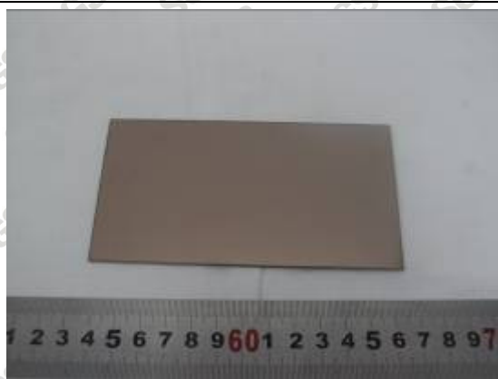
Fig.23 PVD Bronze Colored Stainless Steel Sheets
