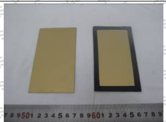
Fig.20 Reference sample Tested sample PVD Gold Colored Stainless Steel Sheets Neutral Salt Spray Test
