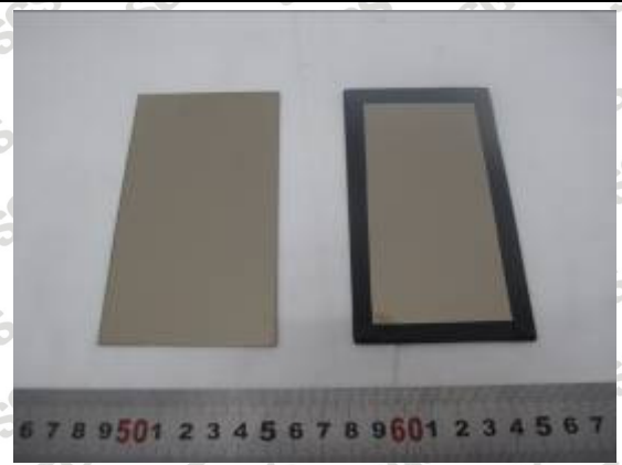
Fig.30 Reference sample Tested sample PVD Nickel Silver Colored Stainless Steel Sheets Neutral Salt Spray Test
