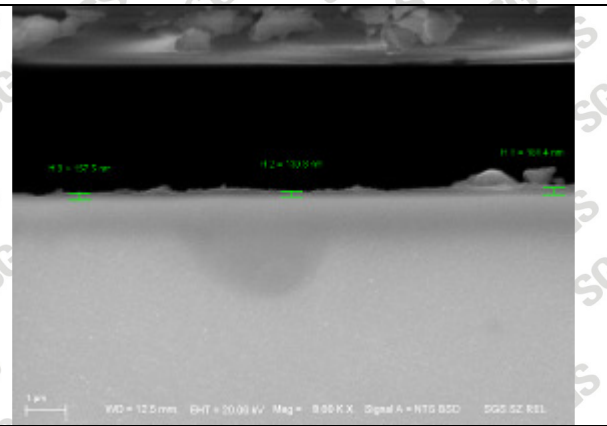
Fig.44 SEM observation –Rose Gold-8000X
