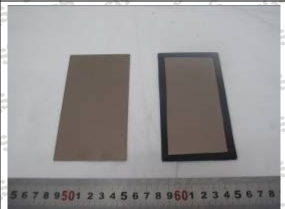
Fig.24 Reference sample Tested sample PVD Bronze Colored Stainless Steel Sheets Neutral Salt Spray Test
