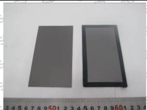
Fig.28 Reference sample Tested sample PVD Black Colored Stainless Steel Sheets Neutral Salt Spray Test
