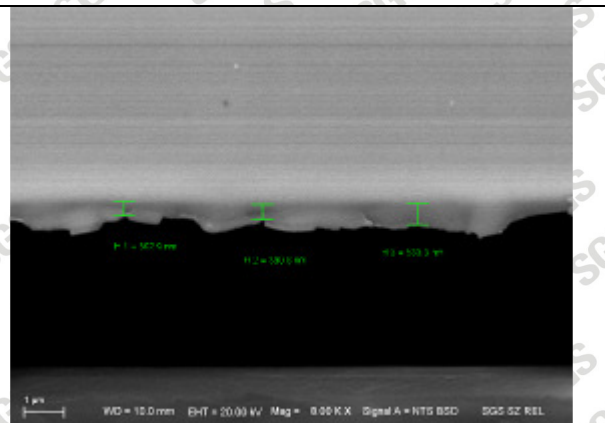
Fig.48 SEM observation – Nickel Silver-8000X
